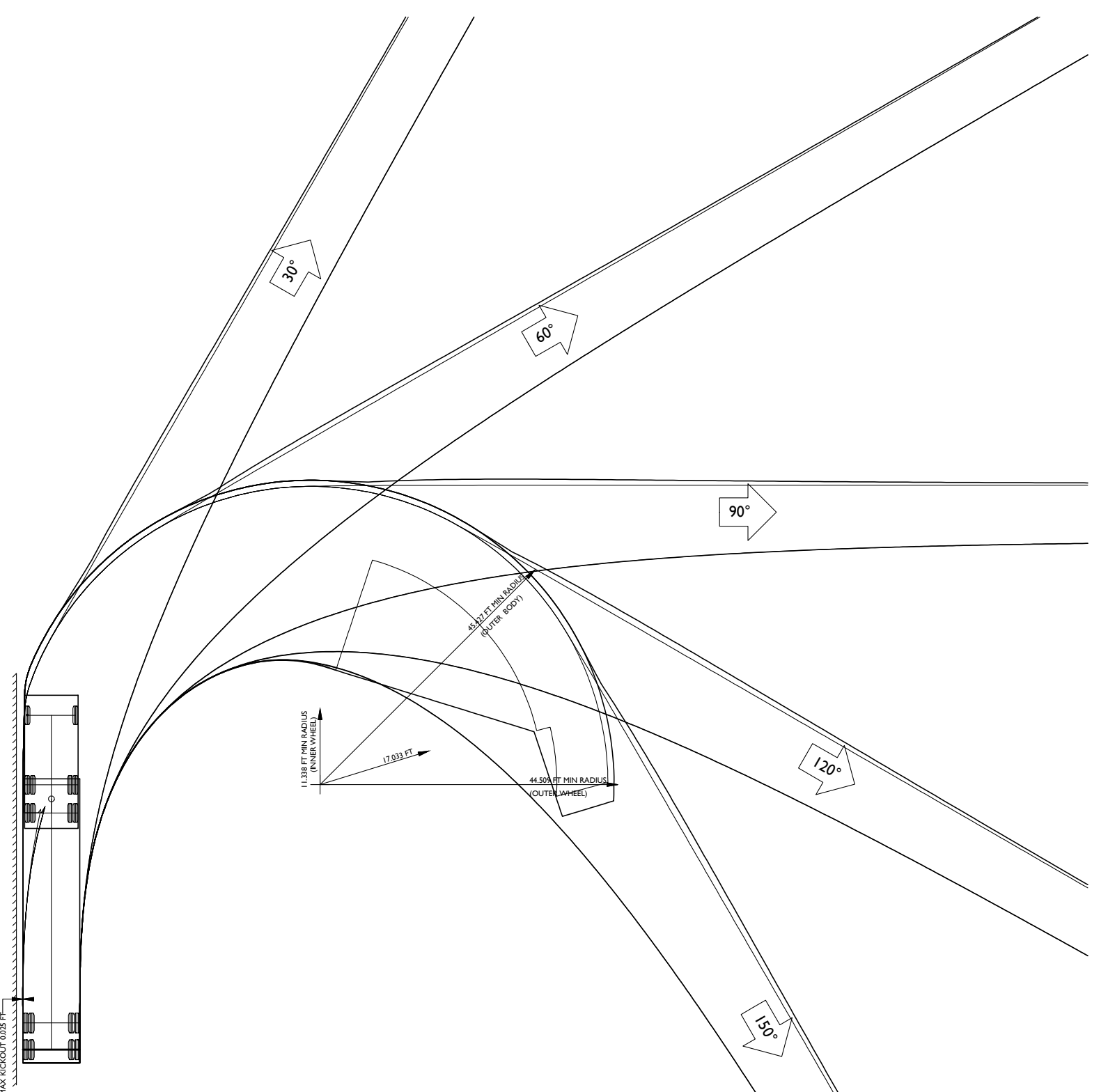
WB-50 - INTERMEDIATE SEMI-TRAILER
