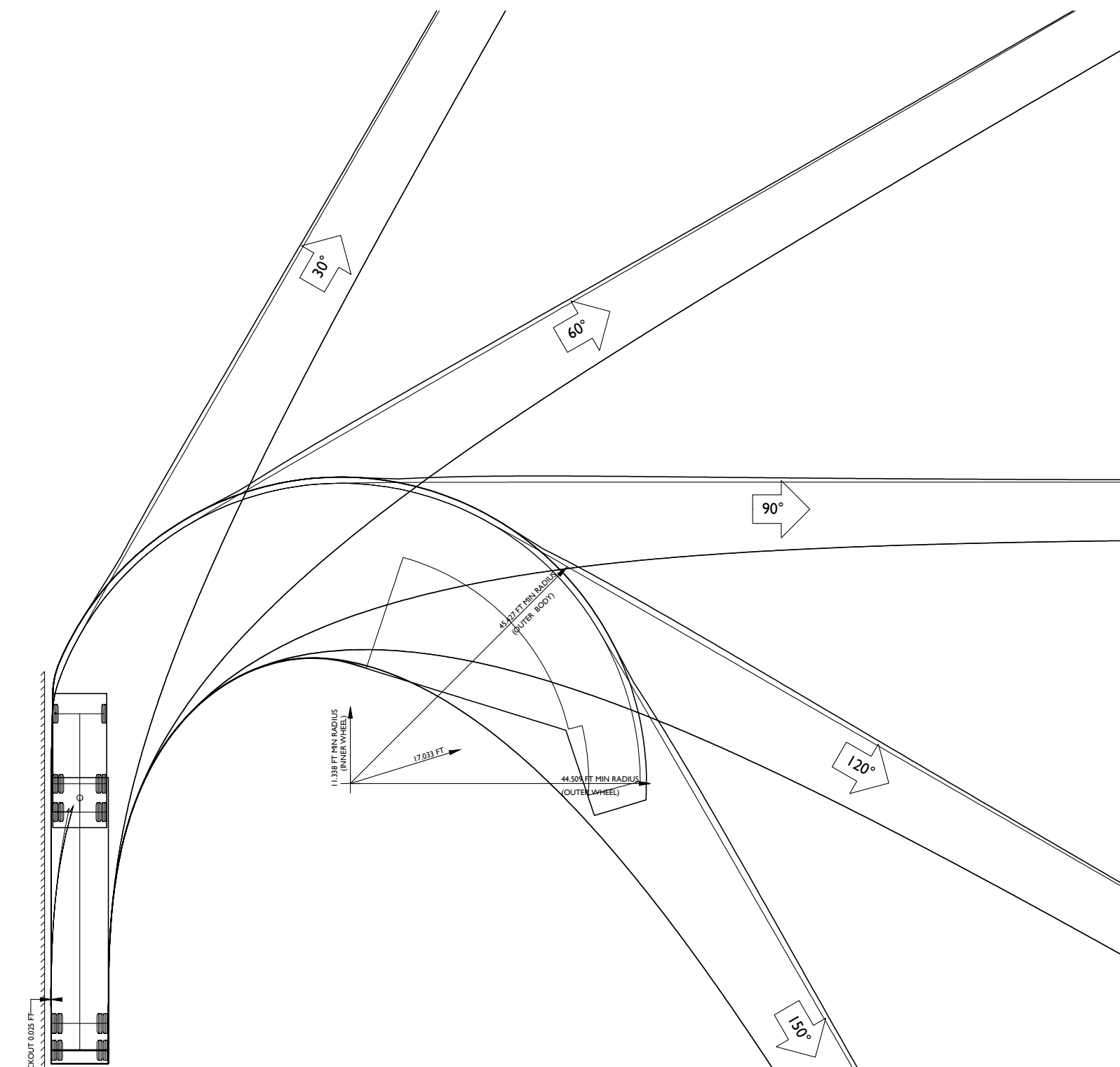
WB-50 - INTERMEDIATE SEMI-TRAILER
