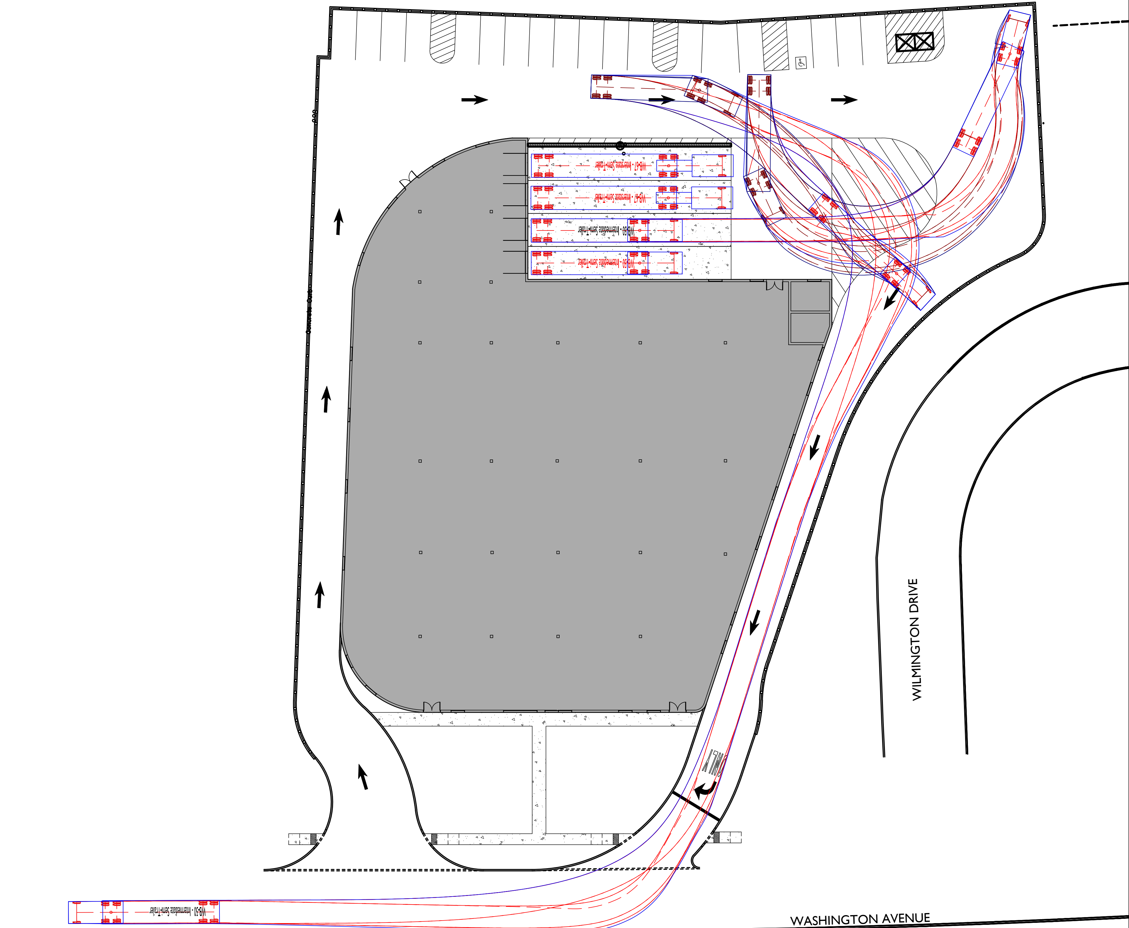
WB-50 - INTERMEDIATE SEMI-TRAILER
